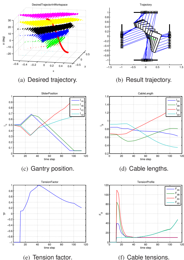
Fig. 8. Reconfiguration to optimize tension factor along trajectory.
