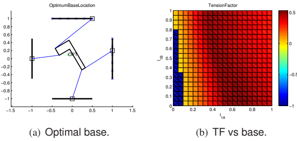
Fig. 7. Effect of base repositioning.
