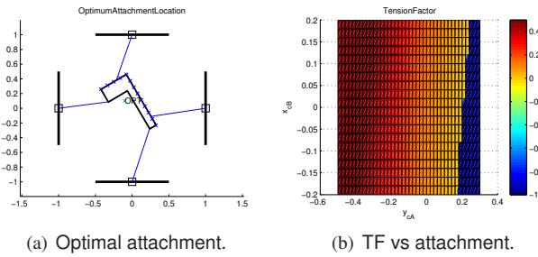
Fig. 6. Effect of cable attachment choice.
