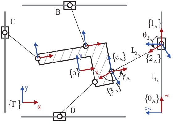
Fig. 3. Payload with 4 Agents(A,B,C,D).
