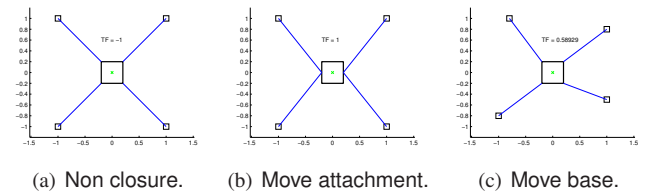
Fig. 5. Simple illustration of reconfiguration.
