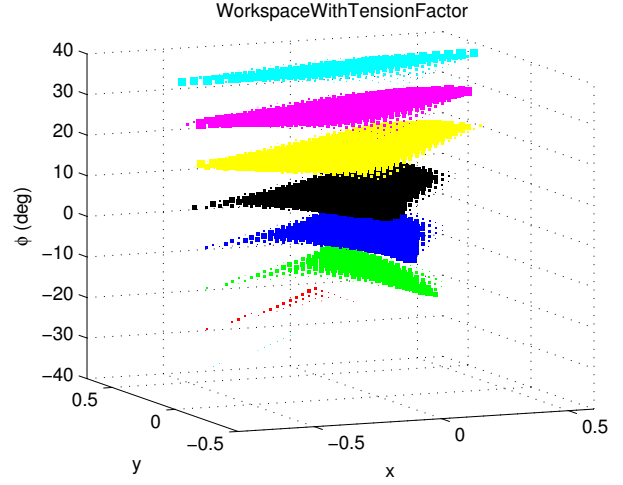
Fig. 4. Workspace tension factor.
